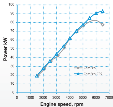
Power Curve
