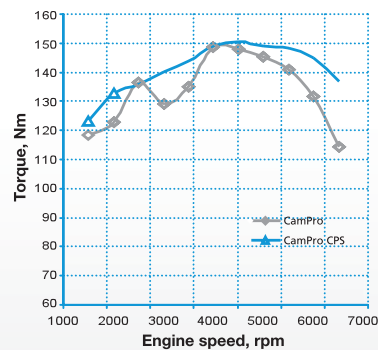
Torque Curve
